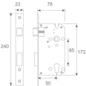
鎖體尺寸 Lock Body size
