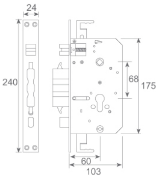
鎖體尺寸 Lock Body size
