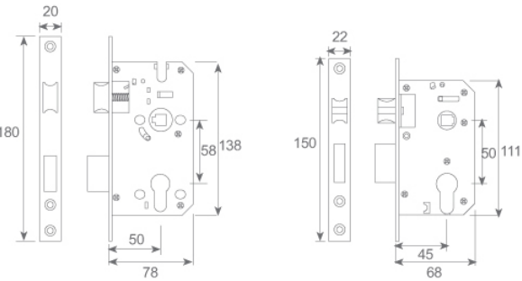
鎖體尺寸 Lock Body size
