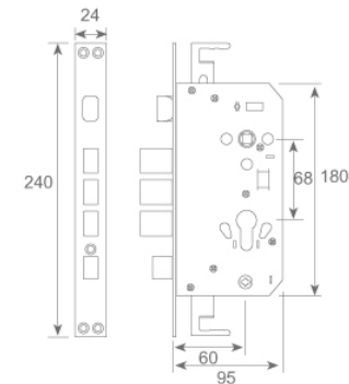
鎖体尺寸 Lock Body size
