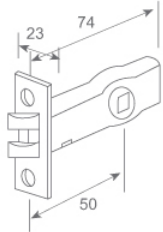
鎖體尺寸 Lock Body size
