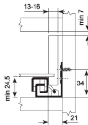
Cabinet Space Arrangement 箱體內空間需求
