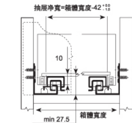
Drawer / Inner Drawer 低抽屜/內低抽
