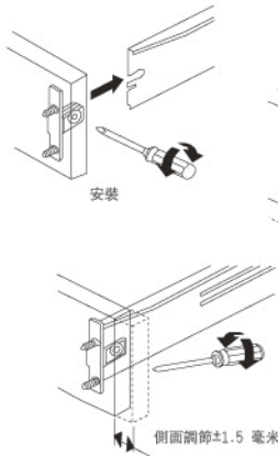
Drawer Panel 抽屜面板
