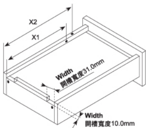
Drawer / Inner Drawer 低抽屜 / 內低抽
