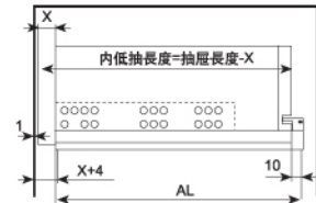
Inner Drawer 內低抽
