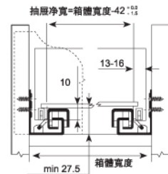
Drawer / Inner Drawer 低抽屜/內低抽
