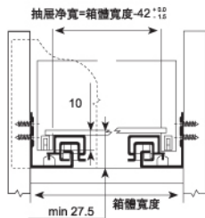
Drawer / Inner Drawer 低抽屜 / 內低抽
