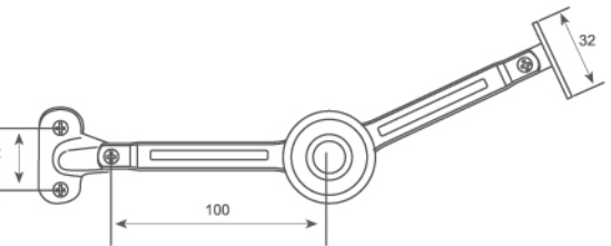
FD-B03-360° Flap Stay 任意停支撑
