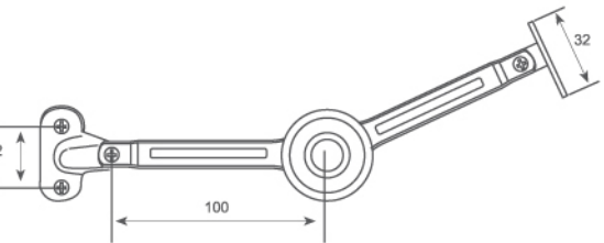
FD-B03 Flap Stay 任意停支撑
