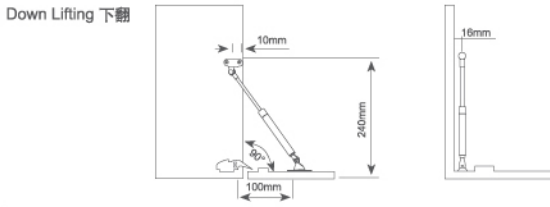
Down Lifting 下翻
